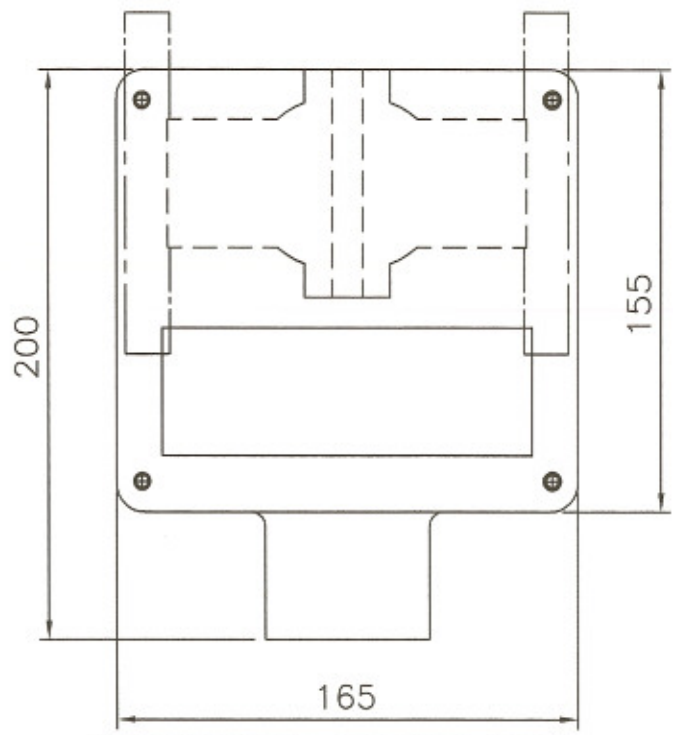
HORIZONTAL FRONT VIEW
